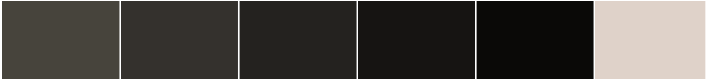
S 4502-Y
