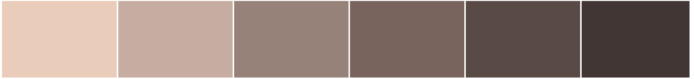
S 0505-Y80R
