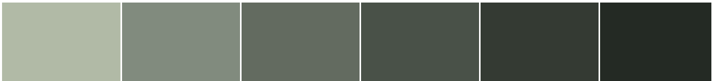
S 1005-G20Y
