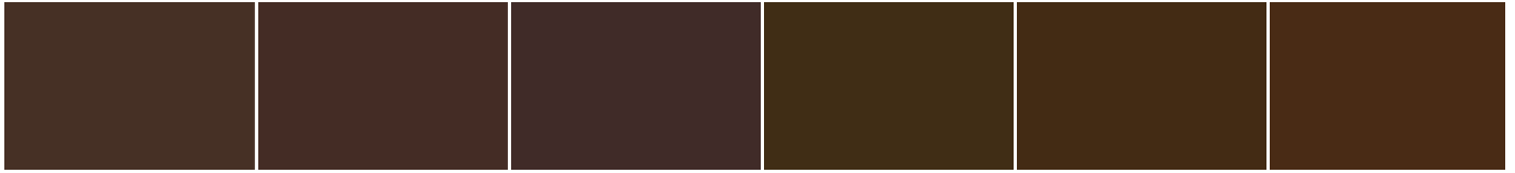
S 5010-Y50R
