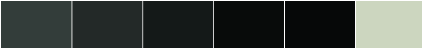
S 5005-B80G
