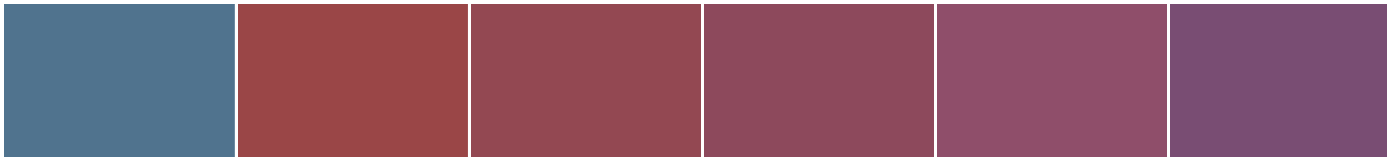
S 2020-R90B
