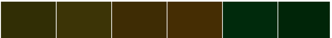
S 4050-G60Y
