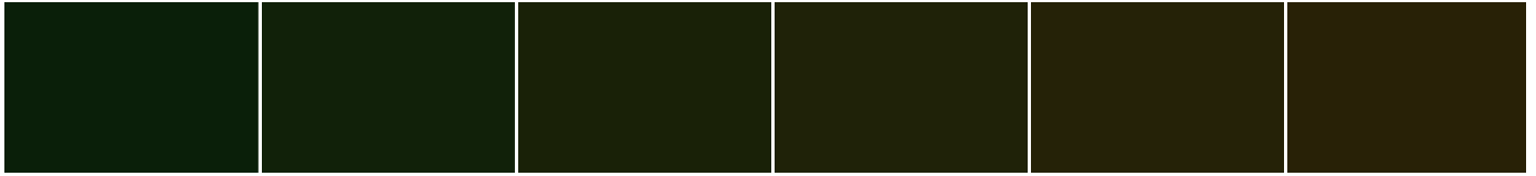
S 5040-G20Y
