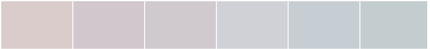
S 0505-R30B
