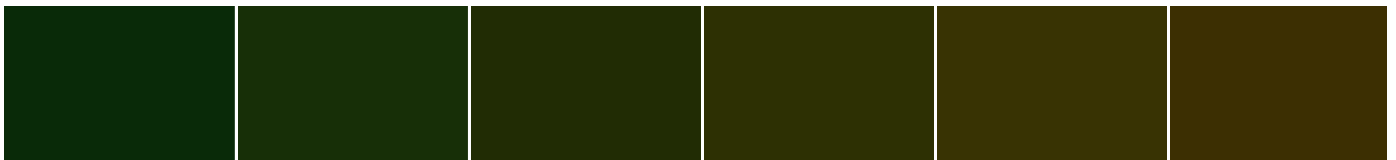
S 3560-G20Y
