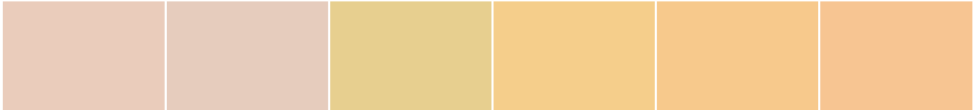
S 0505-Y80R
