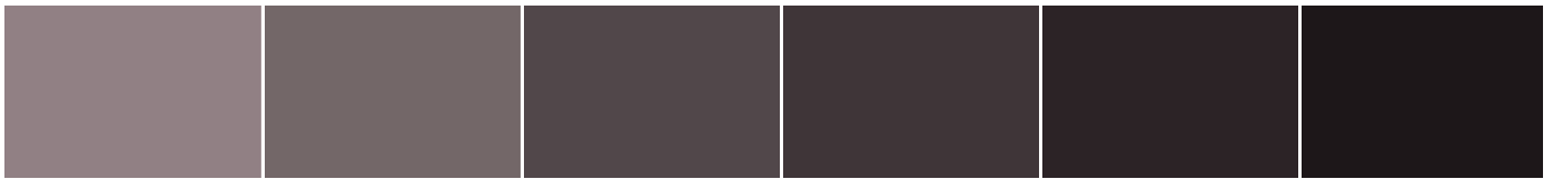
S 2005-R20B
