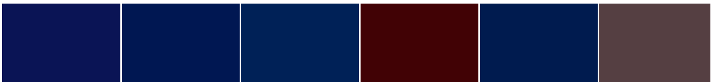
S 3060-R70B
