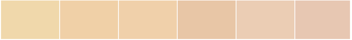
S 0505-Y20R
