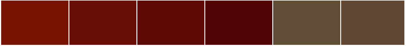
S 2570-Y60R
