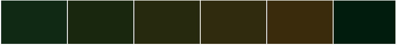
S 5030-G10Y
