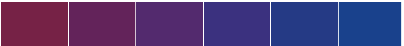
S 2050-R30B
