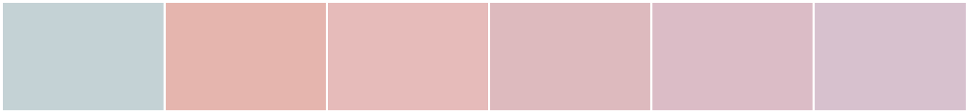
S 0505-R90B
