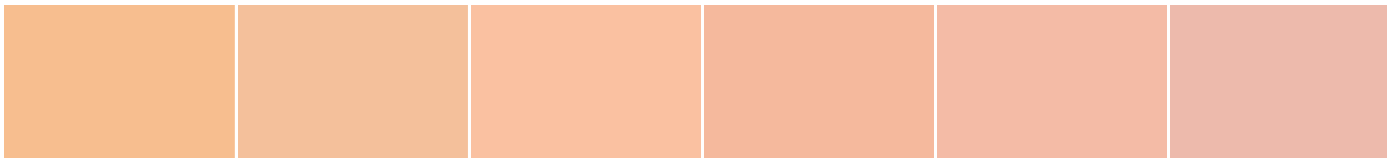
S 0510-Y40R
