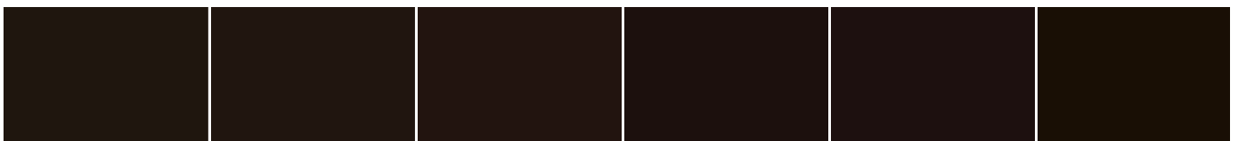
S 7010-Y10R
