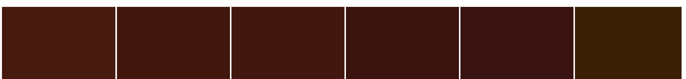
S 5030-Y50R
