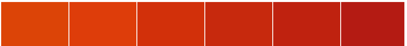
S 1070-Y30R
